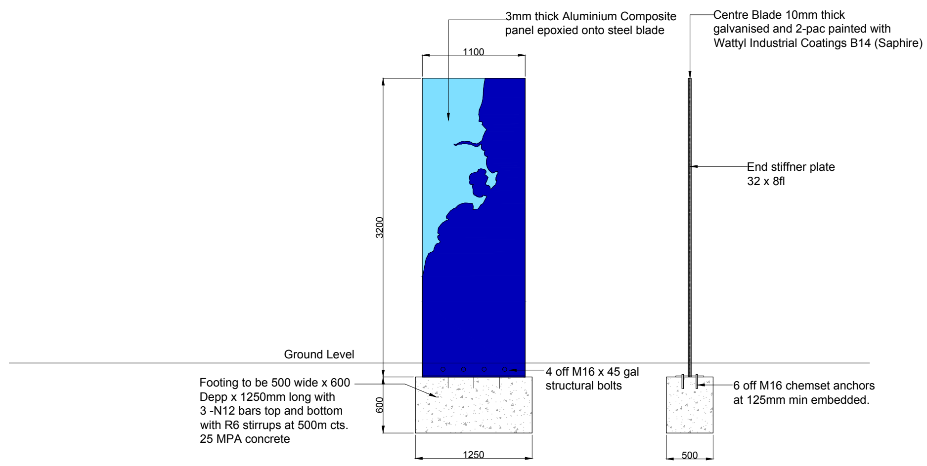
DETAIL: Sign Detail and Footing A1 Scale 1:20 A3 Scale 1:40
